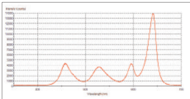
Fig. 10: Spectrum with all LEDs at full.
