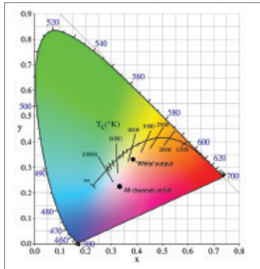
Fig. 9: White points on CIE chart.
