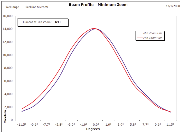
Fig. 8: Output at full.
