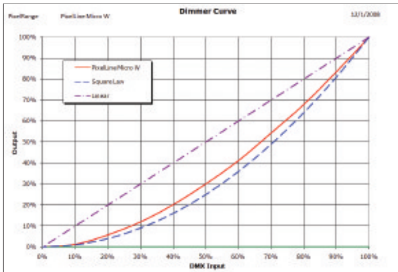
Fig. 12: Dimmer curve.
