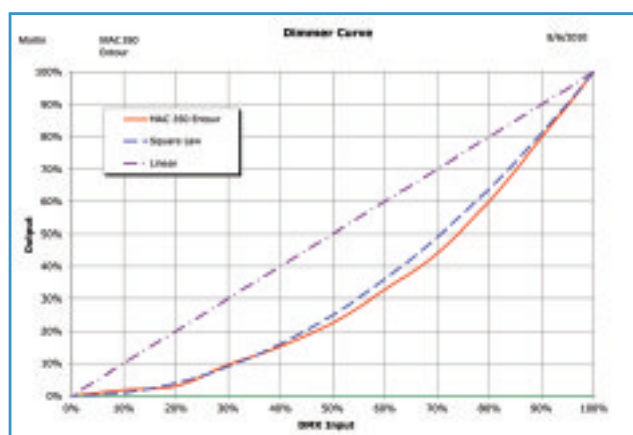
Figure 11 - Dimmer curve
