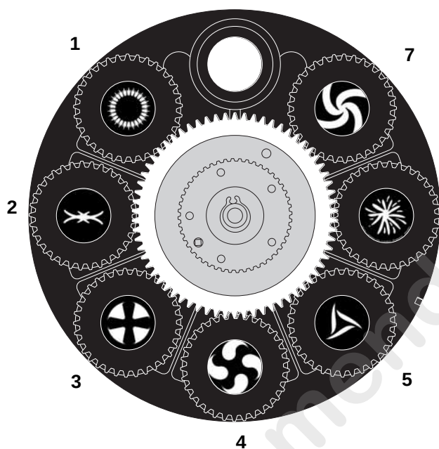
. MAC 250 Krypton rotating gobo wheel
