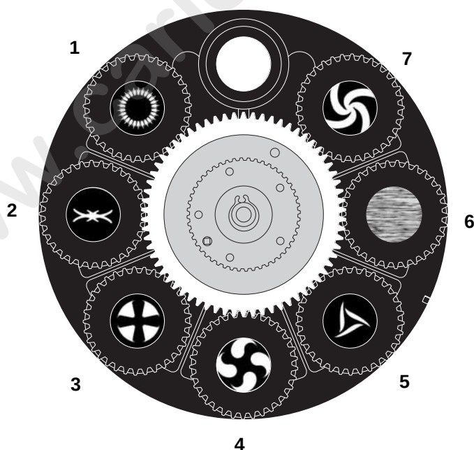
. MAC 250 Entour rotating gobo wheel
