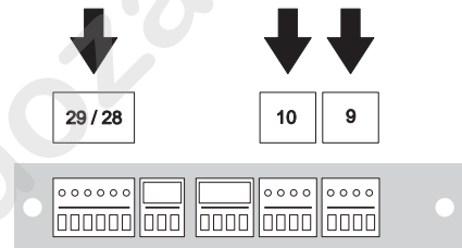
Cable connections
