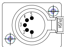
DMX OUT
