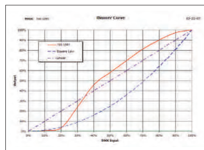
Fig. 6 - Dimmer Law
