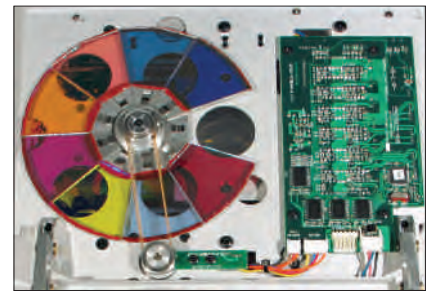
Fig. 8 - Colour wheel
