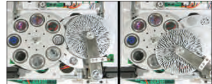
Fig. 9 - Effect wheel
