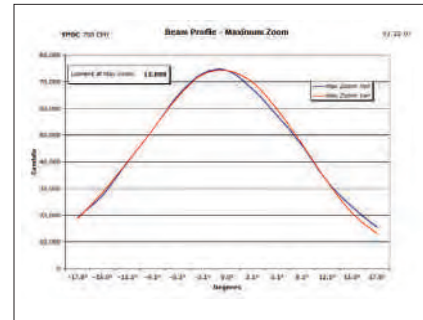
Fig. 17 - Output at wide angle
