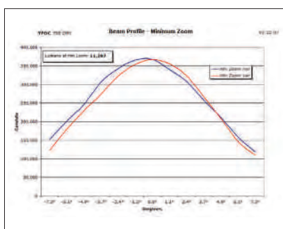
Fig. 16 - Output at narrow angle
