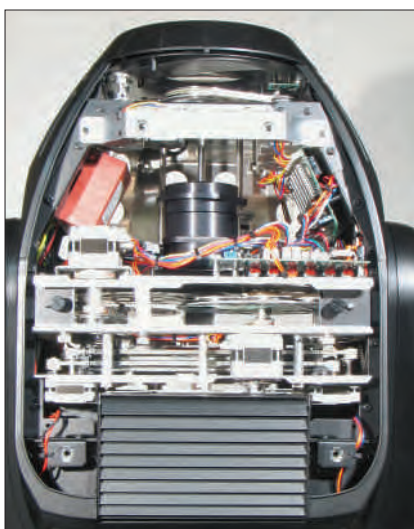
Fig. 14 - Optical bay
