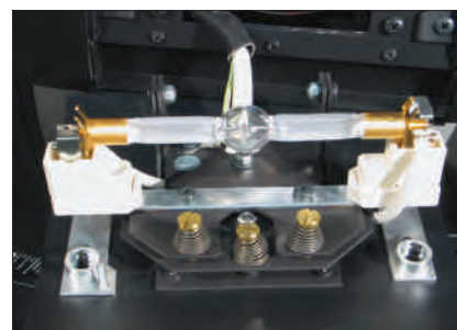
Fig. 3 - Lamp in holder
