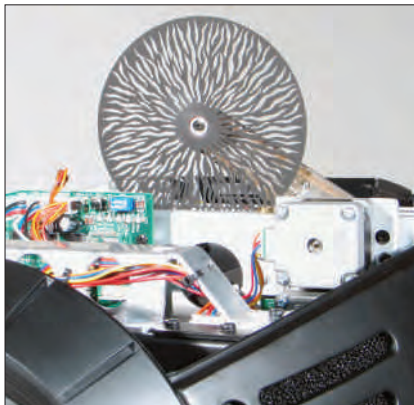
Fig. 11 - Effect wheel change
