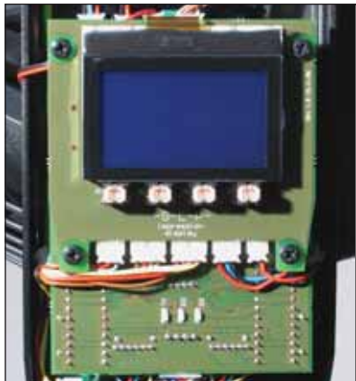
Fig. 12: Display board
