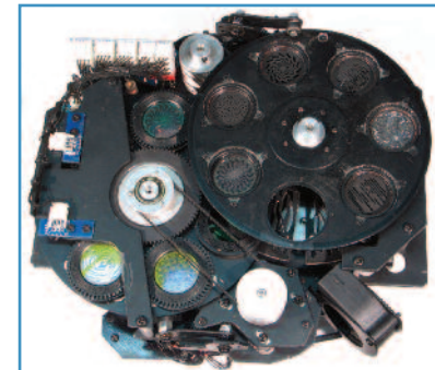
Figure 11 - Gobo module.
