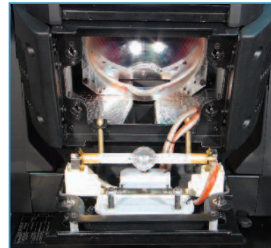
Figure 4 - Lamp house.
