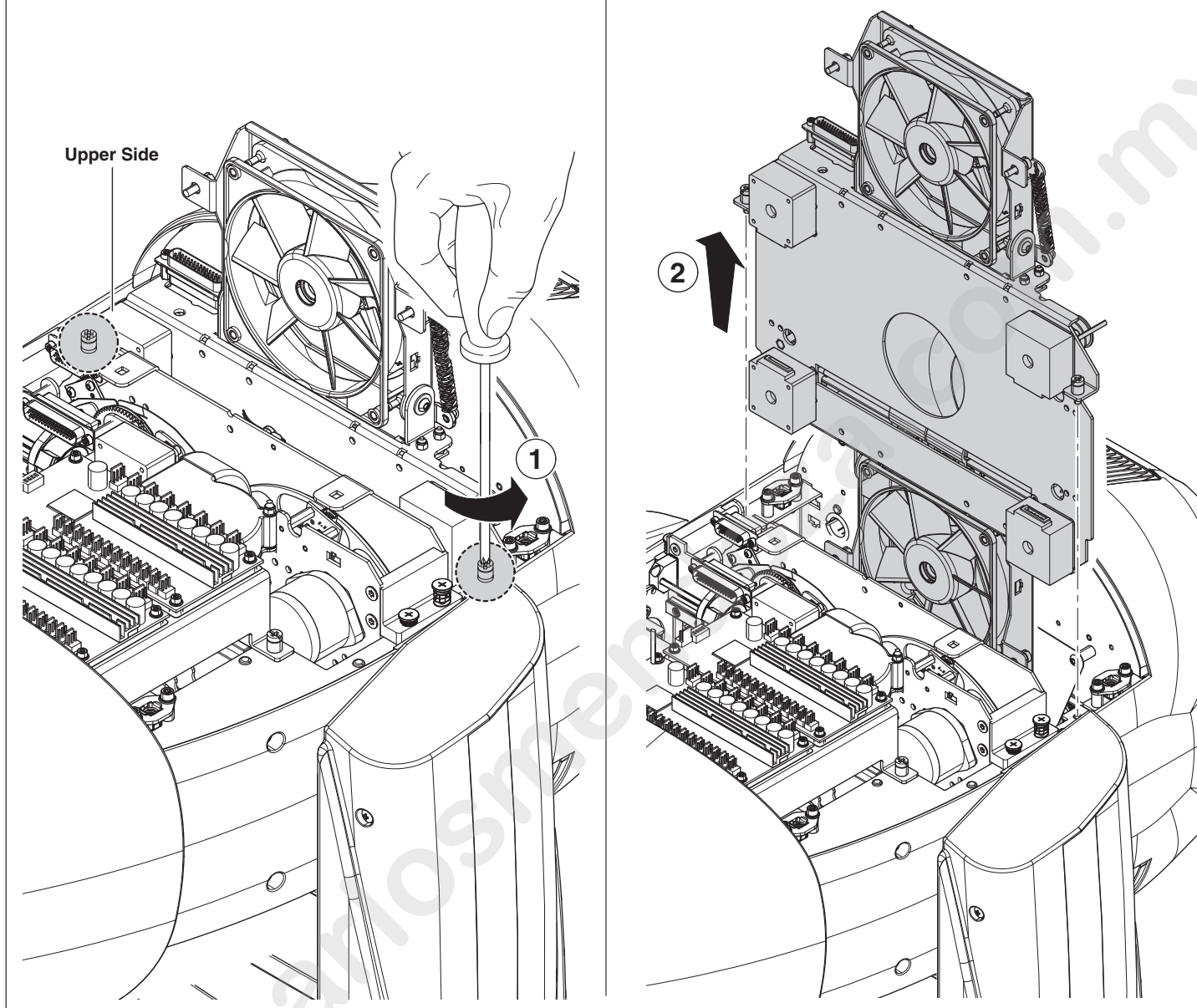
Extraction of the effect modules - Fig. 16.
