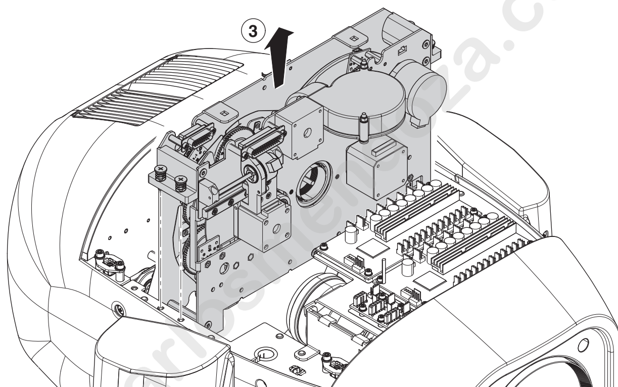
Extraction of the effect modules - Fig. 17.
