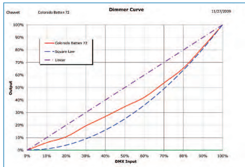
Figure 12: Dimmer curve
