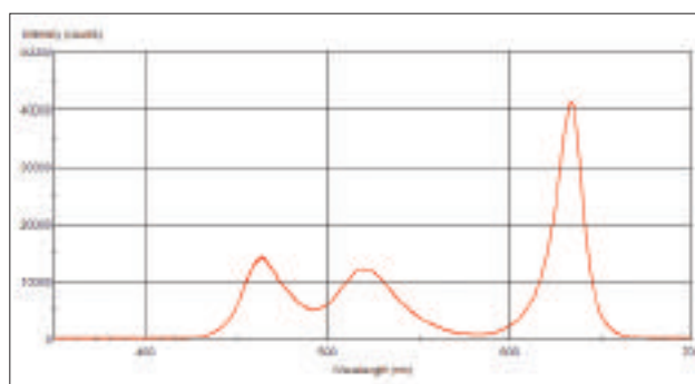
Fig 7: COLORado at full RGB.
