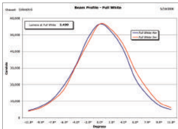
Fig 5: Output in peak white.
