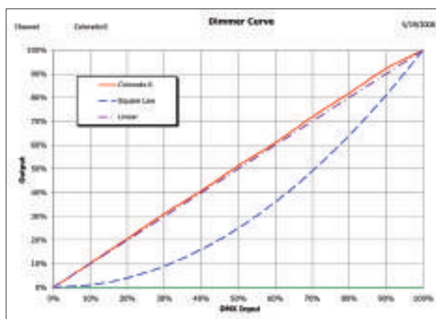
Fig 6: Dimmer Curve.
