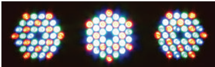
Fig 2: Rotated arrays.
